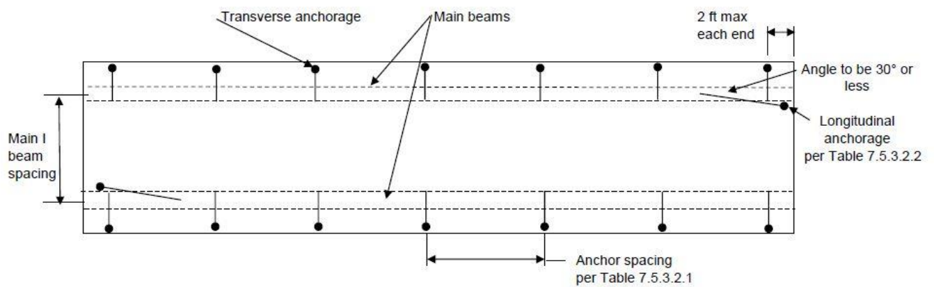
FIGURE 7.5.3.2.1(a) Anchor spacing and location
